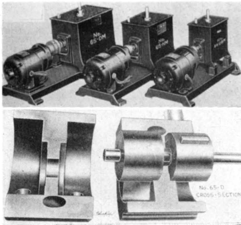
Above: Eisler high-vacuum pumps. Below: Cross-section of the housing of the two-stage high-vacuum pump.
